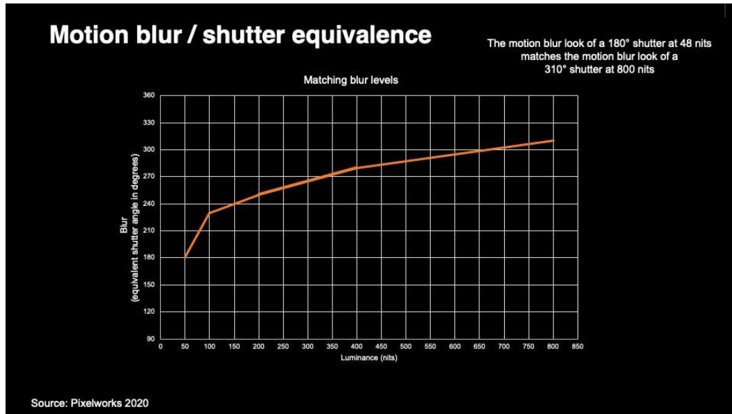
Figure 3: Motion/Blur Model
